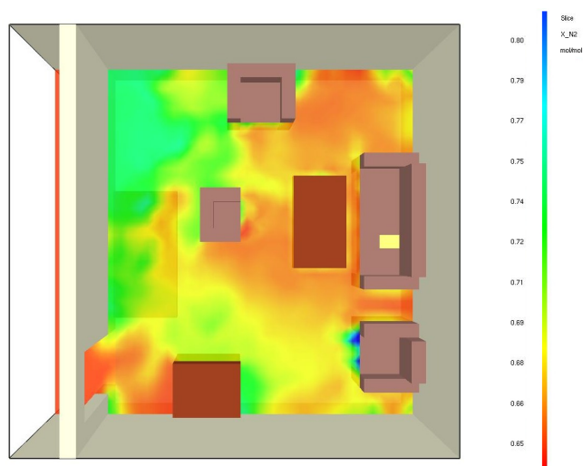
Fig. 1. Example 2D plot of a room with chemical sensor data superimposed. The colour-bar denotes the volume fraction of N_2 in the mixture fraction of other chemical components
