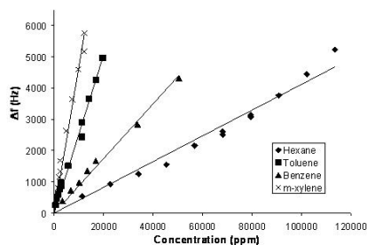
Fig. 3. QCM response to a range of VOC's.
