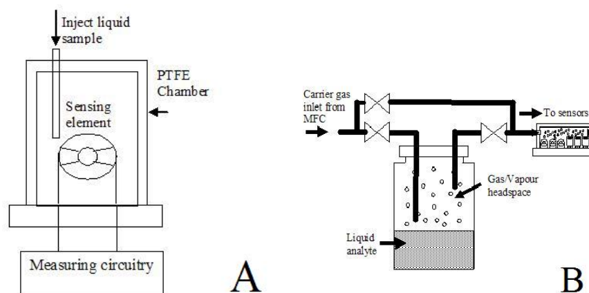
Fig. 2. Basic schematic of Static (A) and Flow (B) basic exposure systems
