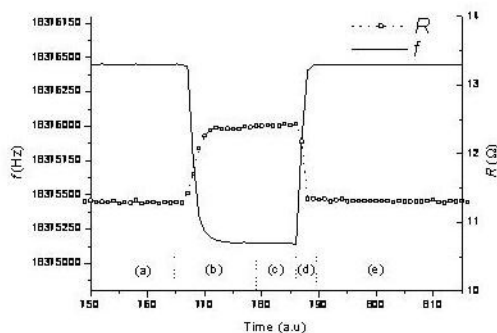
Fig. 5. Dynamic response of a QCM exposed to hexane vapour.
