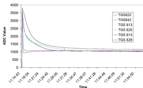
Fig. 4. Startup / initial action of several MOS sensors
