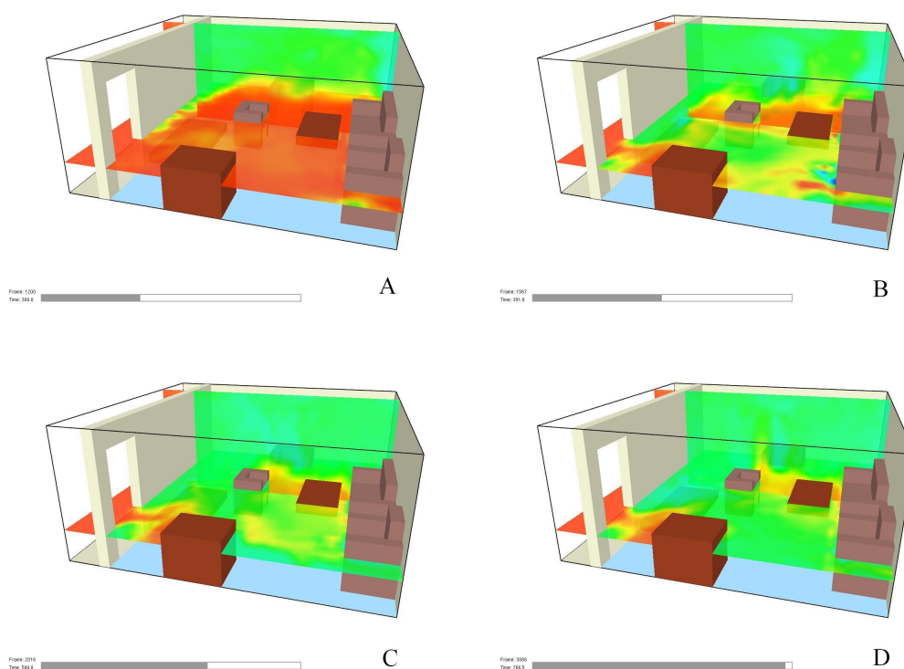
Fig. 6. Snapshots from a polyurethane (foam) fueled fire for horizontal and vertical planes. Note that for clarity only nitrogen concentrations are depicted indicating its dynamic nature. Colour-bar is identical to the one in Figure 1.
